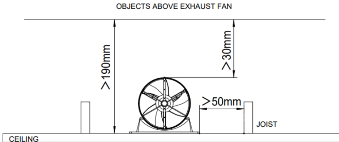
Fig.4 Clearance diagram
