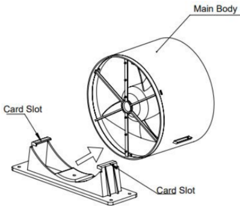
Fig. 1 – Remove main body
