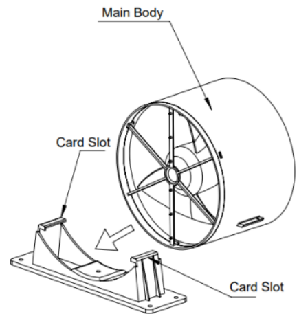
Fig. 3 – Install main body
